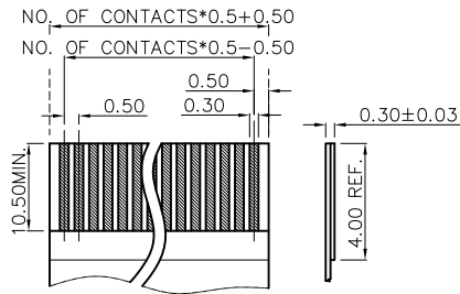
APPLICABLE FPC TOLERANCE: ±0.05
